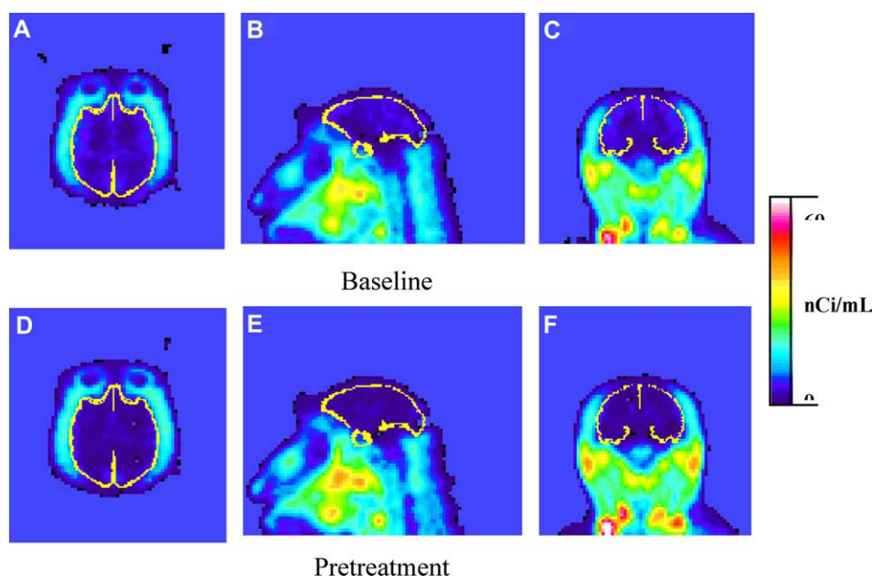
Figure 1. Horizontal (panels A and D), sagittal (panels B and E), and coronal (panels C and F) PET images of cynomolgus monkey head after intravenous injection of NCA [ carbonyl - 11 C]NOWAY in the baseline experiment (panels A–C) and pre-treatment experiment (D–F). Images are from emission data summed from 9 min after injection.
