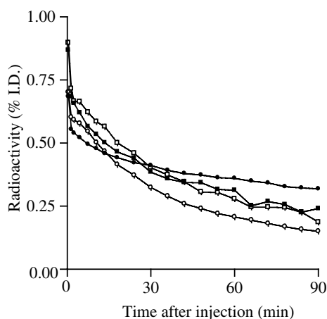
Figure 2. Time courses for radioactivity (% injected dose) in monkey whole brain and cerebellum after injection of NCA [ carbonyl - 11 C] 1 : ● cerebellum in baseline experiment; ○ cerebellum in pre-treatment experiment; ■ whole brain in baseline experiment; □ whole brain in pre-treatment experiment.
